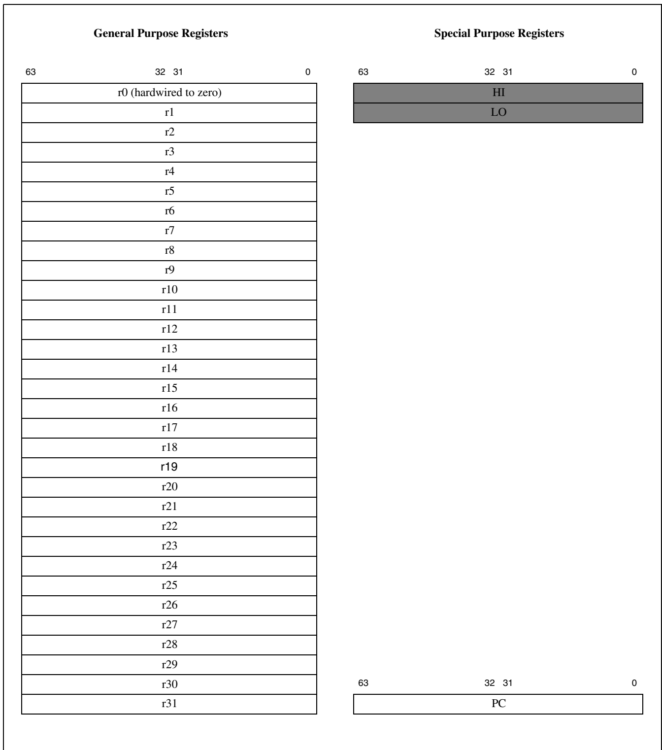
Figure 4.1 CPU Registers for MIPS64
